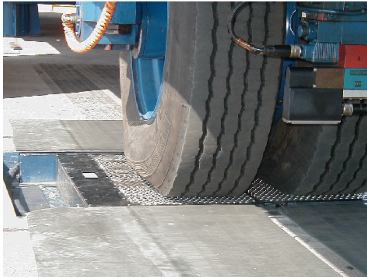
Figure 2: Twin (or dual) SIM pad configuration (used under Heavy Vehicle Simulator (HVS) with dual test tyres).
