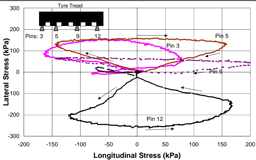
Figure 8: Horizontal shear stress excursion for four sensors: Tyre 35 kN, 720 kPa
