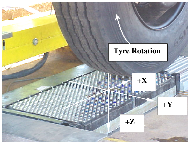
Figure 4: SAE sign convention used during SIM measurements. X-Longitudinal, Y-Lateral and Z Vertical loads/stresses.
